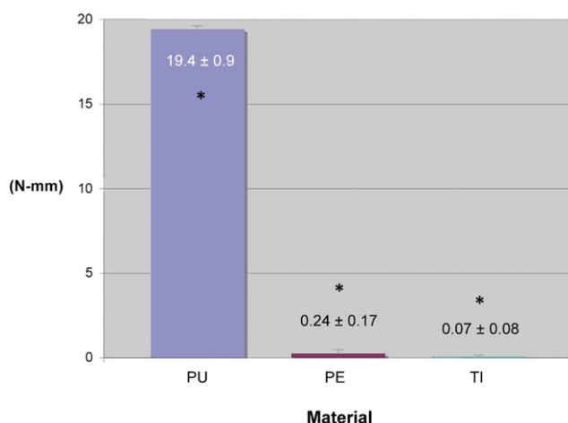
Fig. 4. Plot of viscous damping ratio for each group of nucleus materials ( n = 10 each). The value in newton-millimeters is included for each material, along with the standard deviation. An asterisk indicates that a group is statistically different from the other groups.
