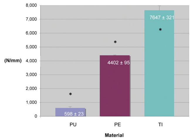
Fig. 5. Plot of dynamic stiffness for each group of nucleus materials ( n = 10 each). The value in newtons per millimeter is included for each group, along with the standard deviation. An asterisk indicates that a group is statistically different from the other groups.
