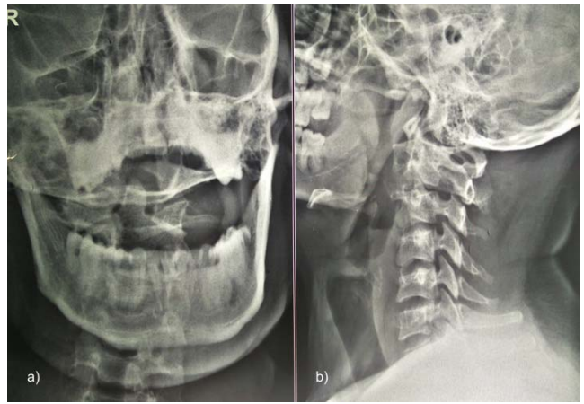
Figure 3. Preoperative x-ray: (a) Note eccentric position of the odontoid. (b) Lateral x-ray showing rotation at C1-2 with elliptical appearance of the C1 arch.
