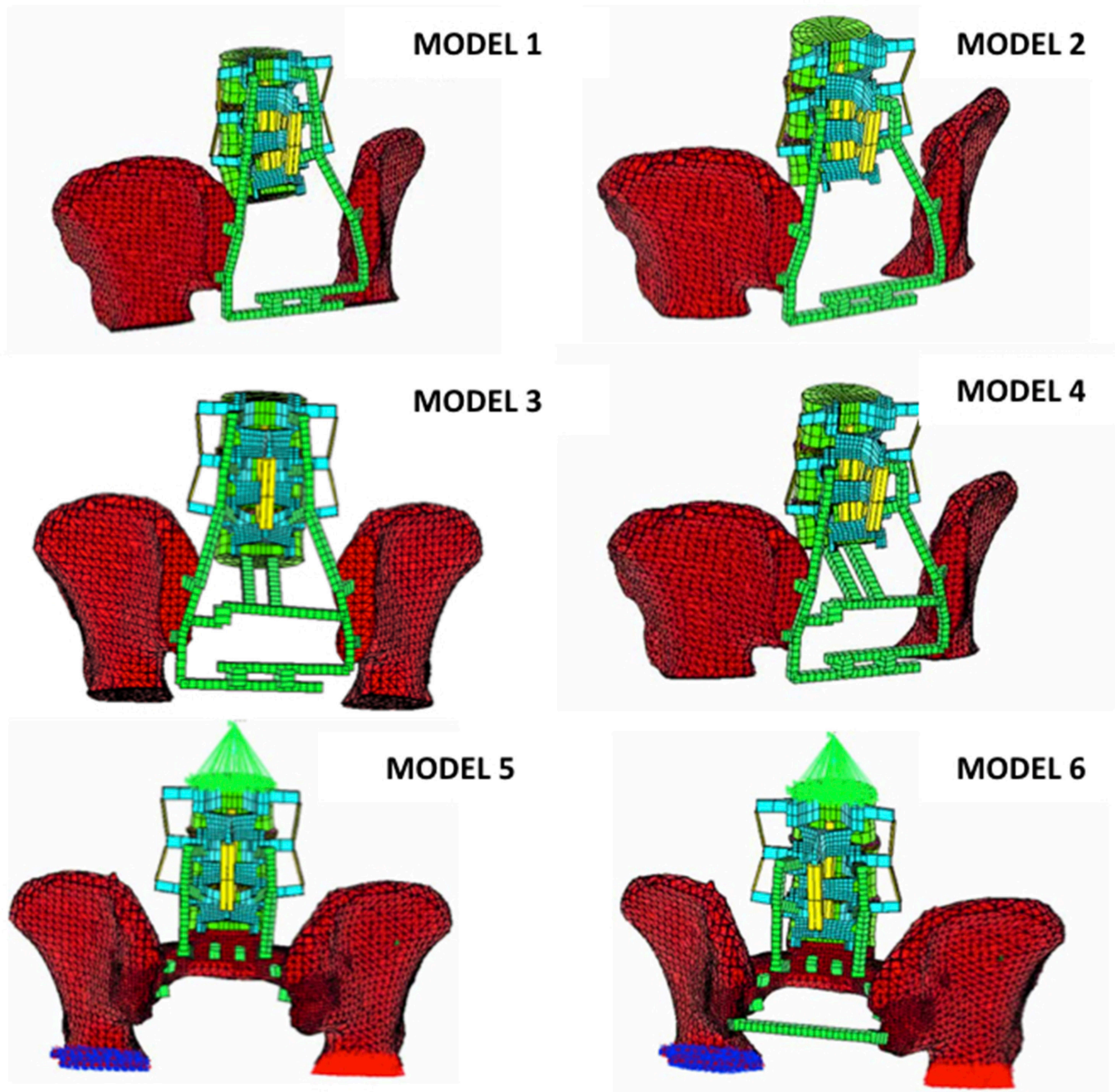
Figure 3. Finite element models.
