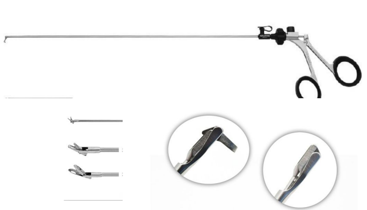
Fig. 16. Endoscopic instruments shown. Illustrations show a 1 hook, 2 articulated graspers for targeting migrated fragments and 3 a back biter amongst others.
