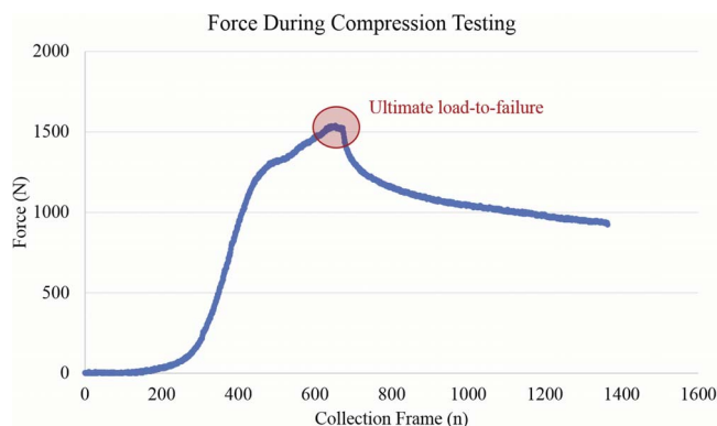
Figure 4. Representative load to failure as defined on force output from compression data.
