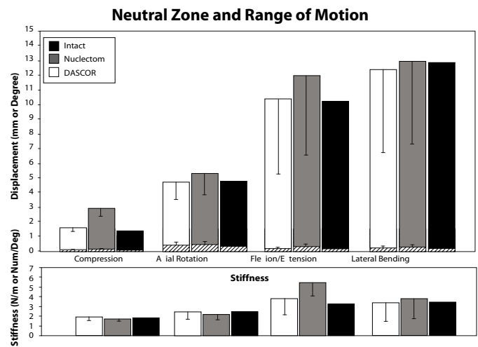
A figure depicting the multidirectional flexibility results comparing the intact, nucleotomy, and nucleus replacement device segmental constructs. The graph on top presents the results obtained for neutral zone (crossed line bars within solid shaded bars) and range of motion. The bottom graph presents results obtained for segmental stiffness. Error bars reflect one standard deviation.
