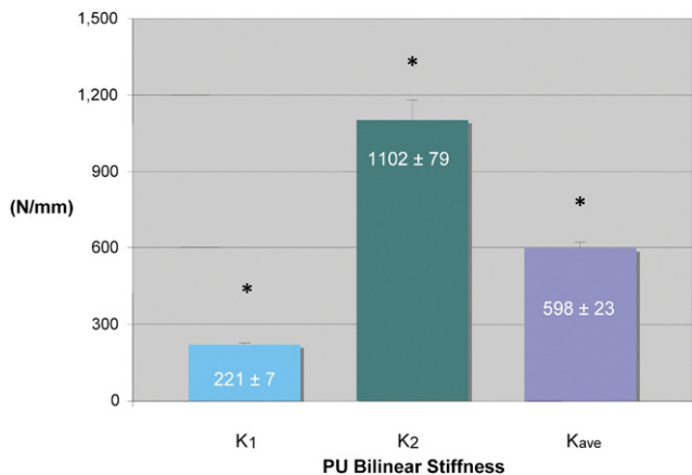
Fig. 7. Plot of initial ( K_1 ), secondary ( K_2 ), and average ( K_{ave} ) quasi-static stiffness for PU nuclei ( n = 10 ). The value in newtons per millimeter is included for each group, along with the standard deviation. An asterisk indicates that a group is statistically different from the other groups.
