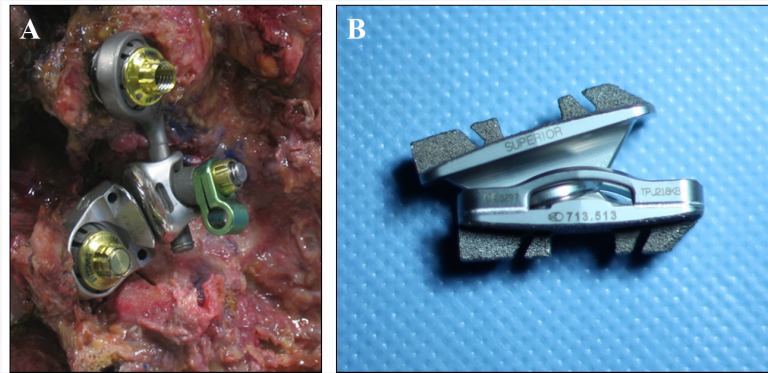
Fig. 1. Images of the facet (A) and posterior total disc (B) replacement devices.
