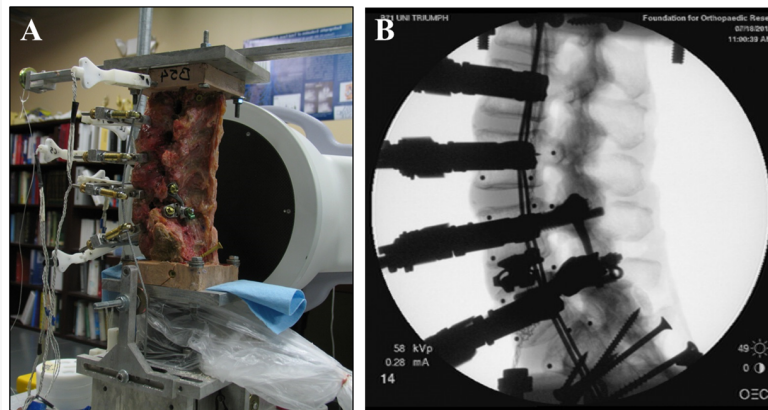
Fig. 2. Biomechanical testing set up showing moment application rod (A) attached at cranial potting and 400N follower load (A, B) using cable guides, steel cables and dead weights (not shown in figure).
